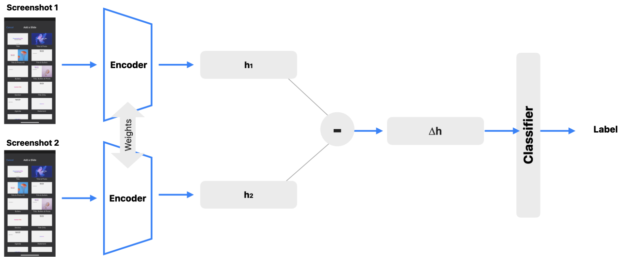
Figure 6: Screen transition model that classifies the transition type between two screens. Two screenshots are featurized using a CNN-based encoder. The resulting embedding vectors ( h_1, h_2 ) are subtracted from each other to produce a difference vector \Delta h , which is used to predict transition type.
